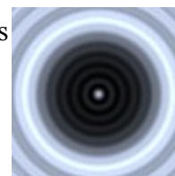
Illustration 1: The Poisson Spot.
