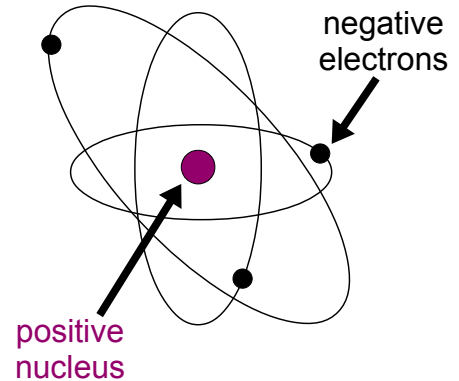
Illustration 3: Rutherford's Nuclear Model.
